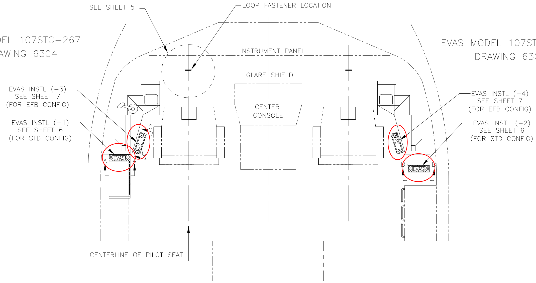
VIEW LOOKING DOWN COCKPIT EVAS INSTL
