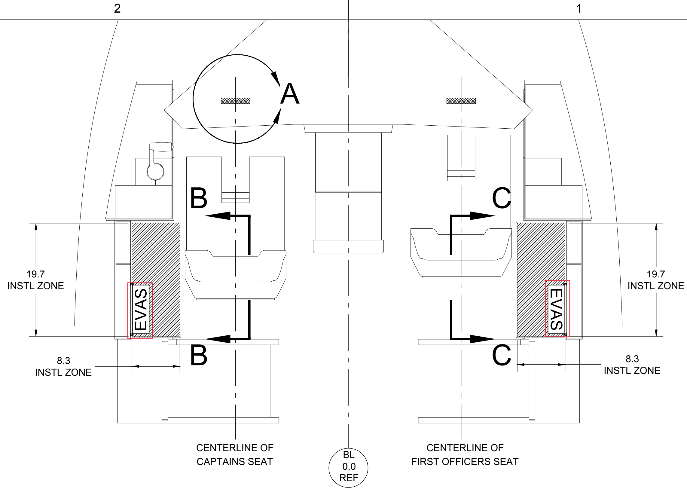
-1 INSTALL, LH, EVAS VIEW LOOKING DOWN
